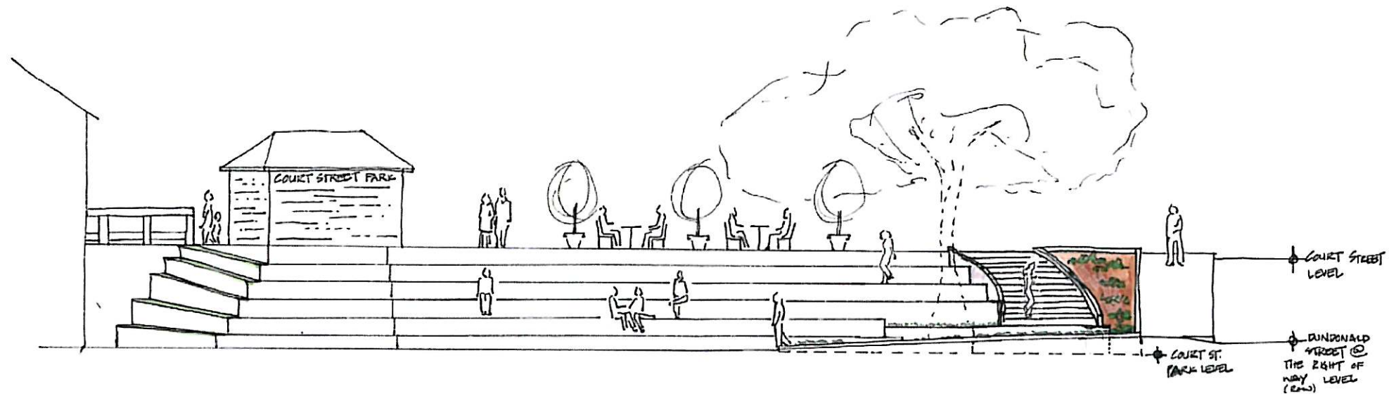
COURT STREET PARK ELEVATION FROM R.O.W. 1/8"
